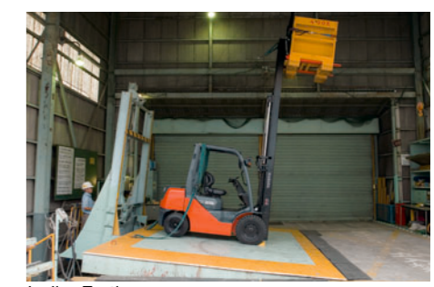
Incline Testing
